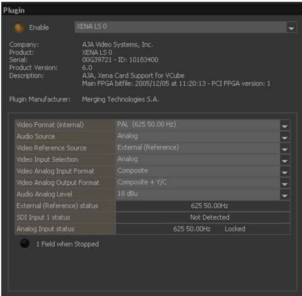
AJA Xena SD and Xena LS Plug-in
