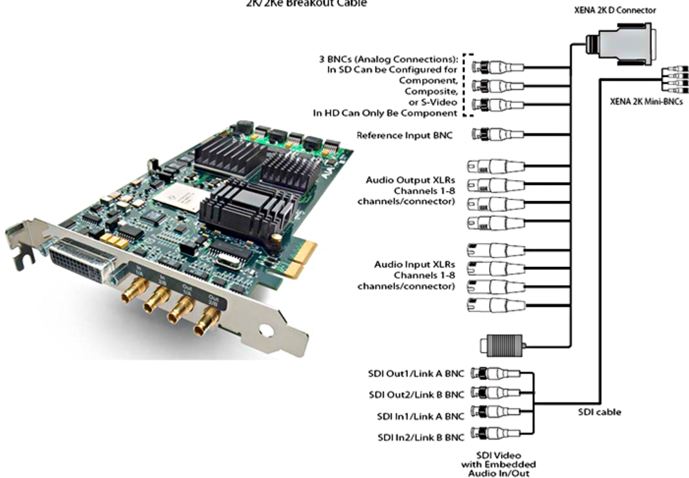
2K/2Ke Breakout Cable
